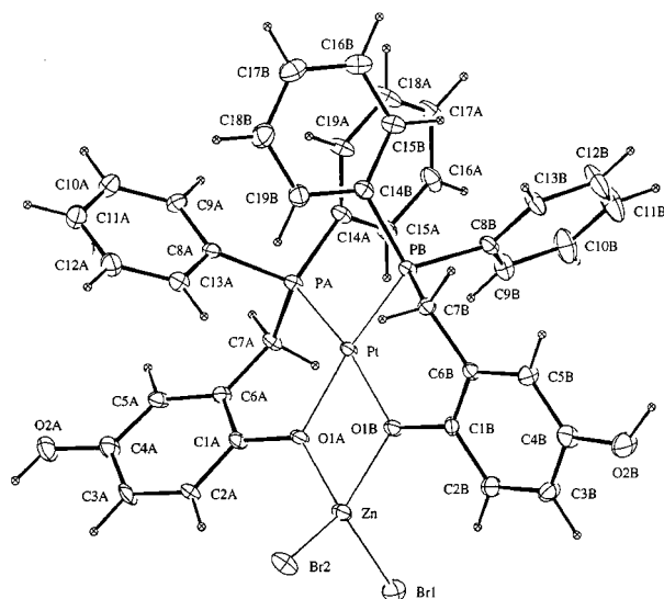
Fig. 3 An ORTEP plot of cis -[Pt(O, P -PPH 2 thqH) 2 (ZnBr 2 )] 2 5 . Details as in Fig. 1.
